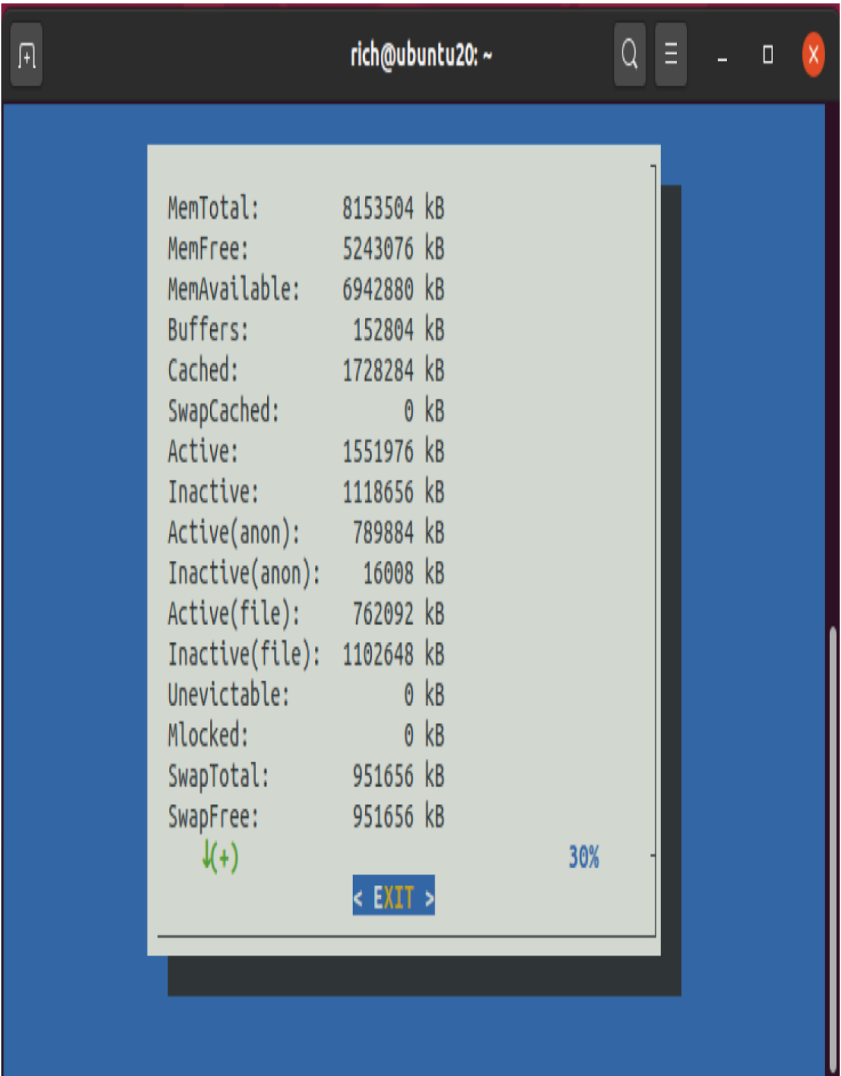
FIGURE 18-8 The meminfo command output displayed using the textbox dialog option
