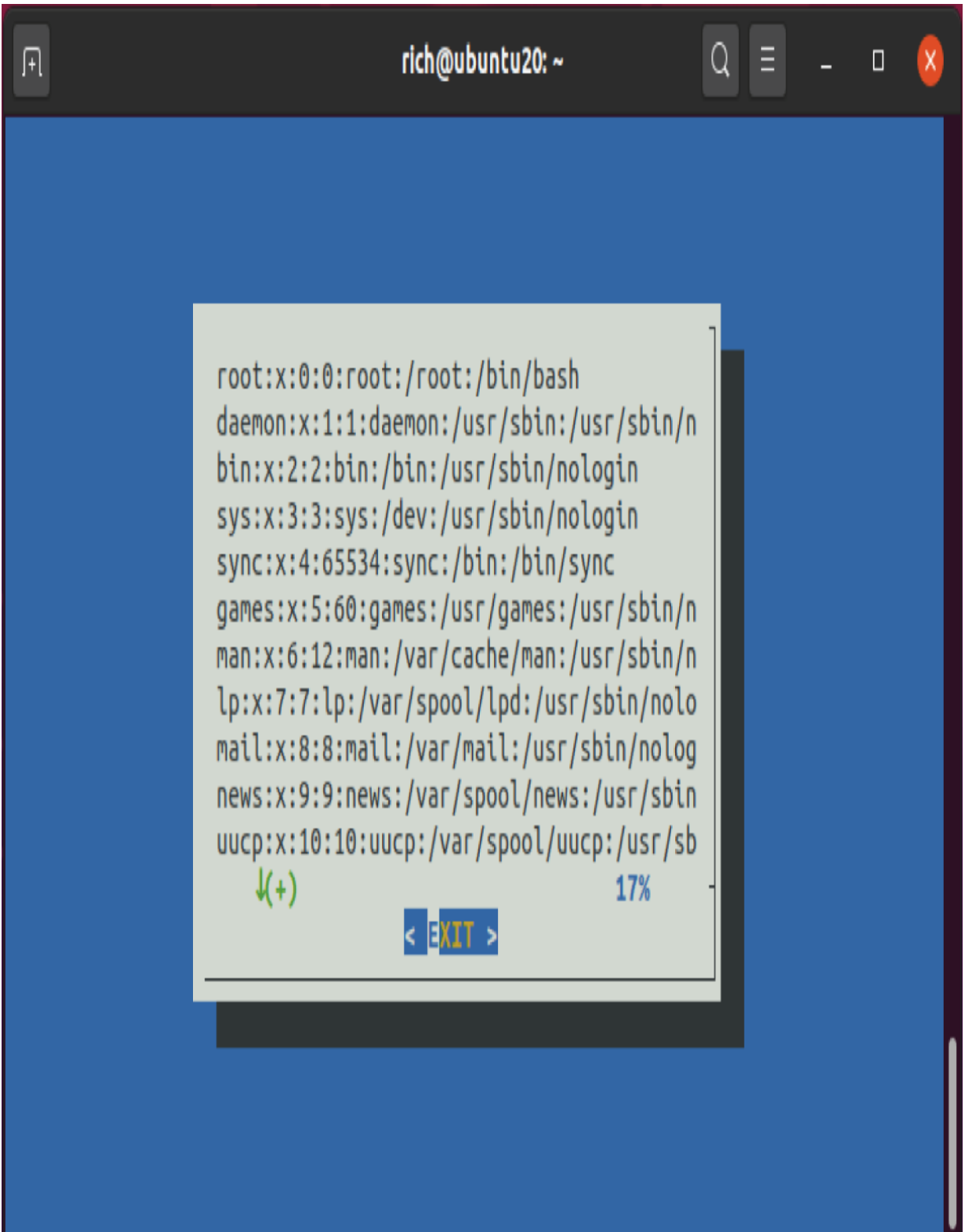
FIGURE 18-5 The textbox widget
