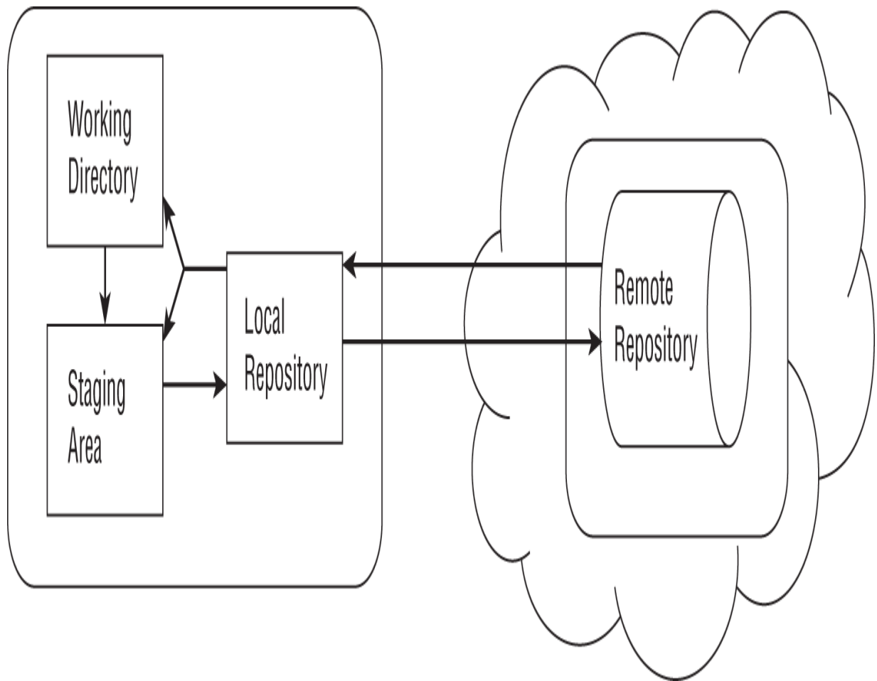
FIGURE 25-1 Conceptual depiction of the Git environment
