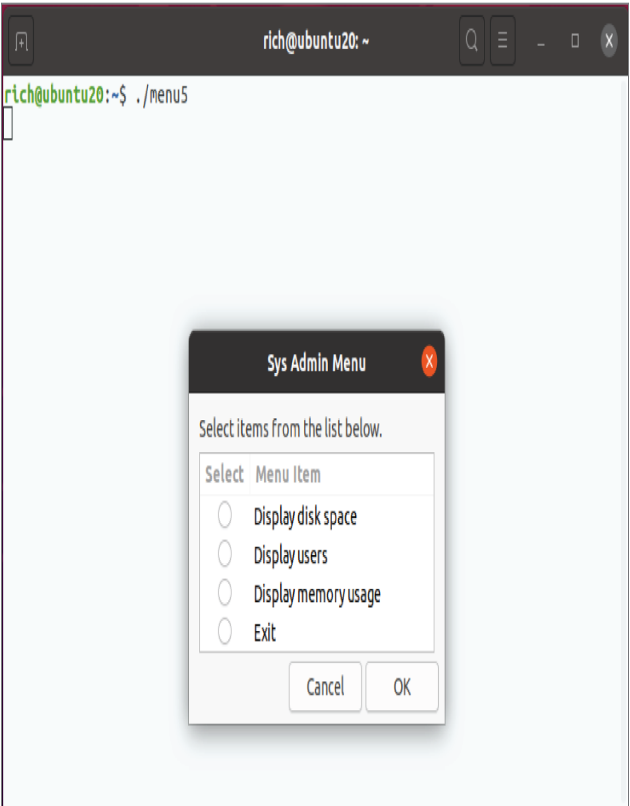
FIGURE 18-13 The system admin menu using zenity
