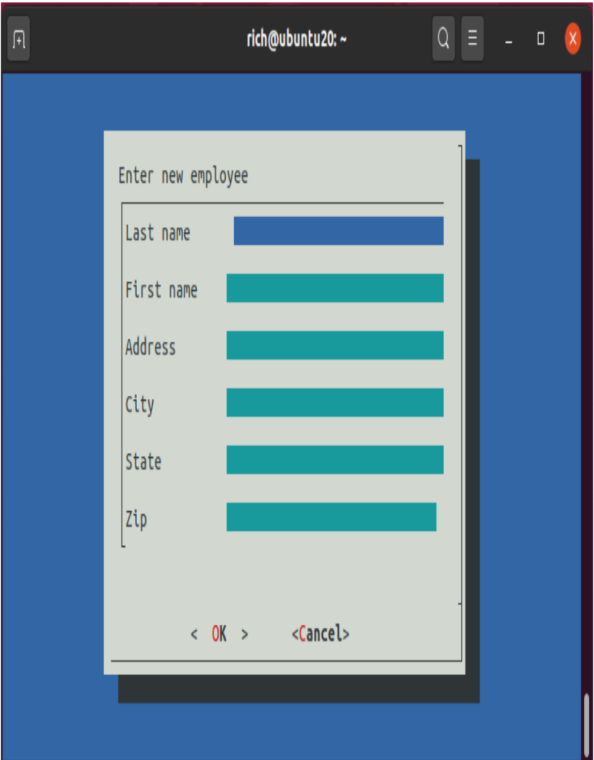
FIGURE 18-14 The dialog form feature
