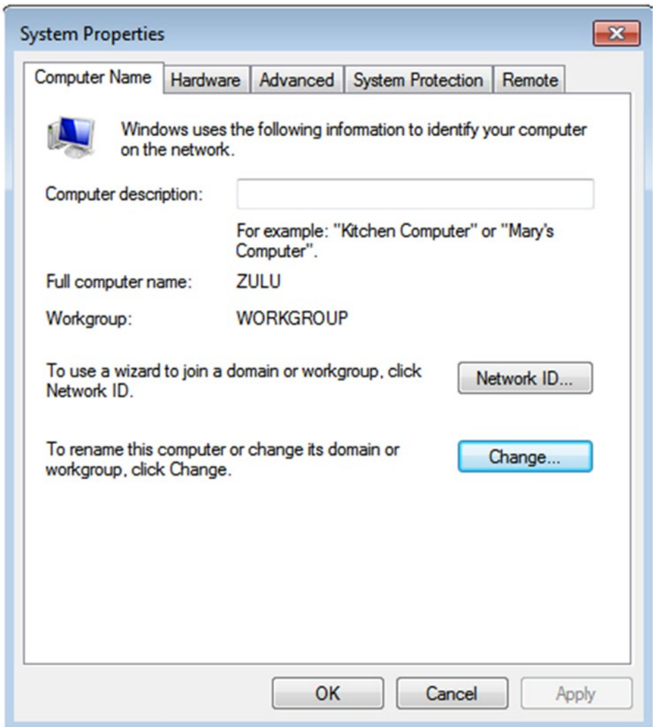
Figure 15-2. System settings
