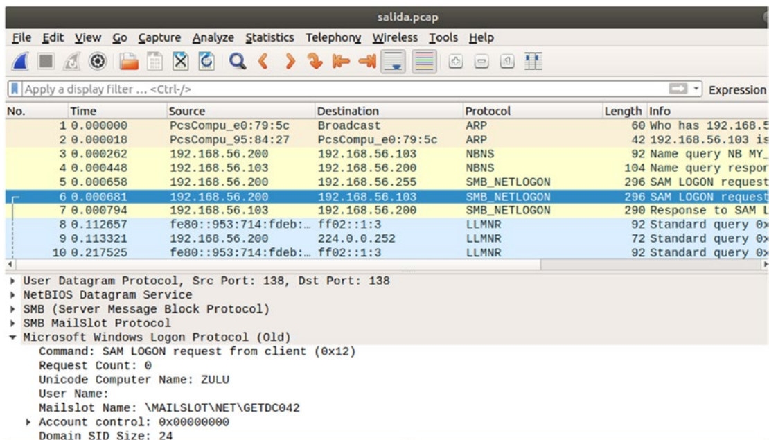
Figure 19-3. Logon request
