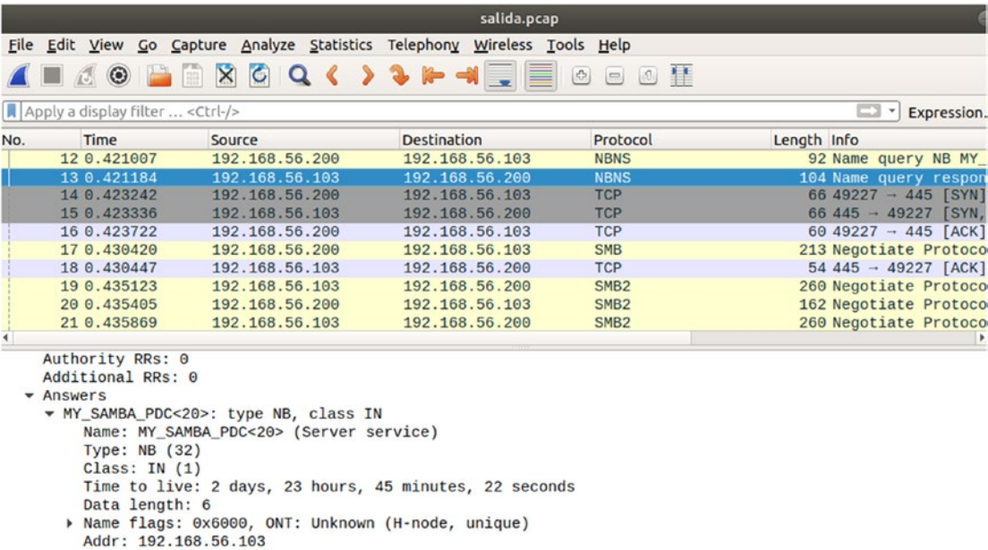
Figure 19-6. NetBIOS response
