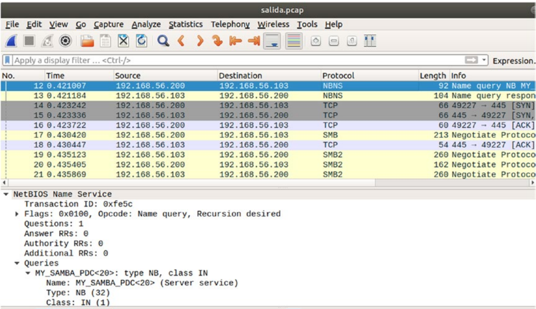
Figure 19-5. Querying the NetBIOS name service again
