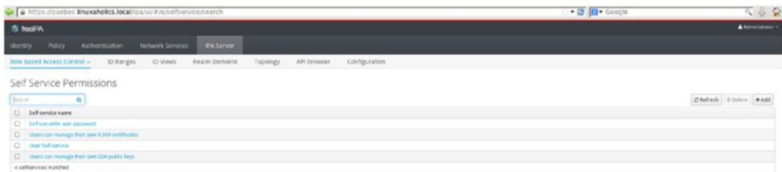
Figure 25-6. Self-service rules
