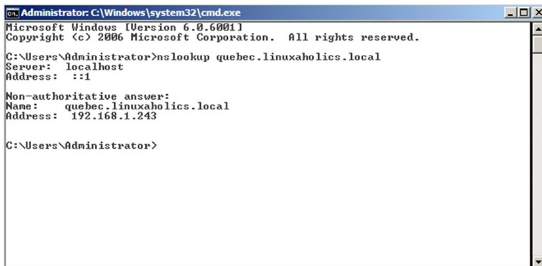
Figure 26-3. Resolving names
