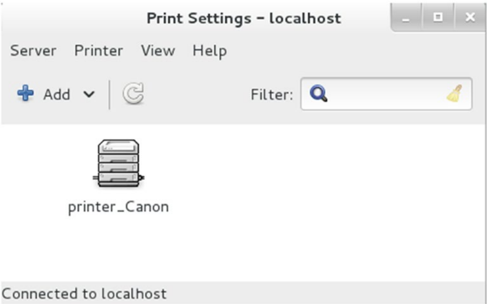
Figure 12-1. system-config-printer
