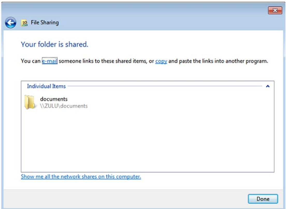
Figure 22-7. Shared resource
