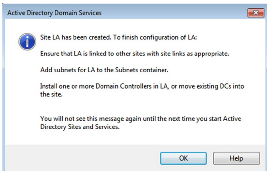
Figure 17-21. Site created
